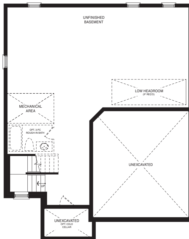
BASEMENT PLAN STYLE A
