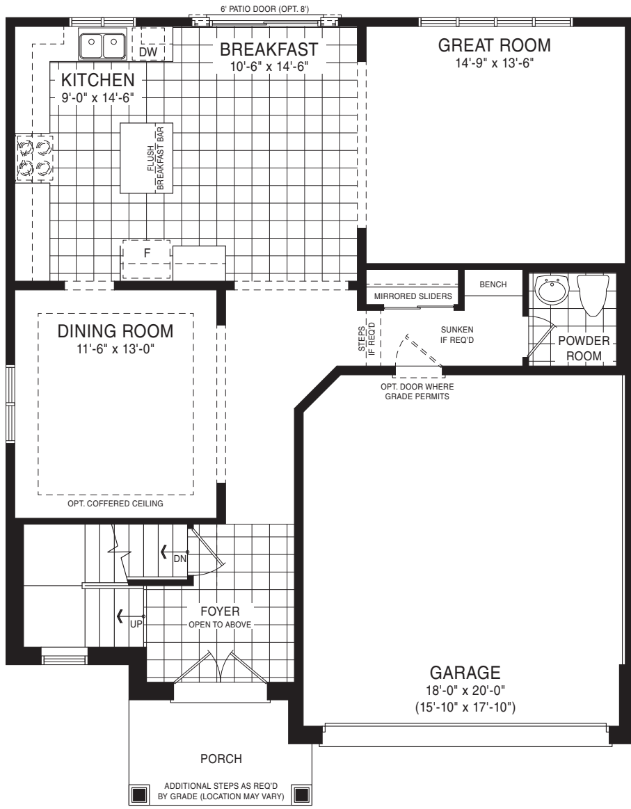
MAIN FLOOR PLAN STYLE A
