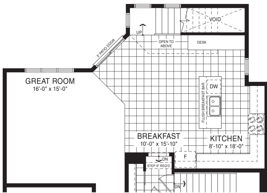
ALTERNATE MAIN FLOOR PLAN - ALT-2A STYLE A
