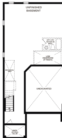
BASEMENT PLAN STYLE A
