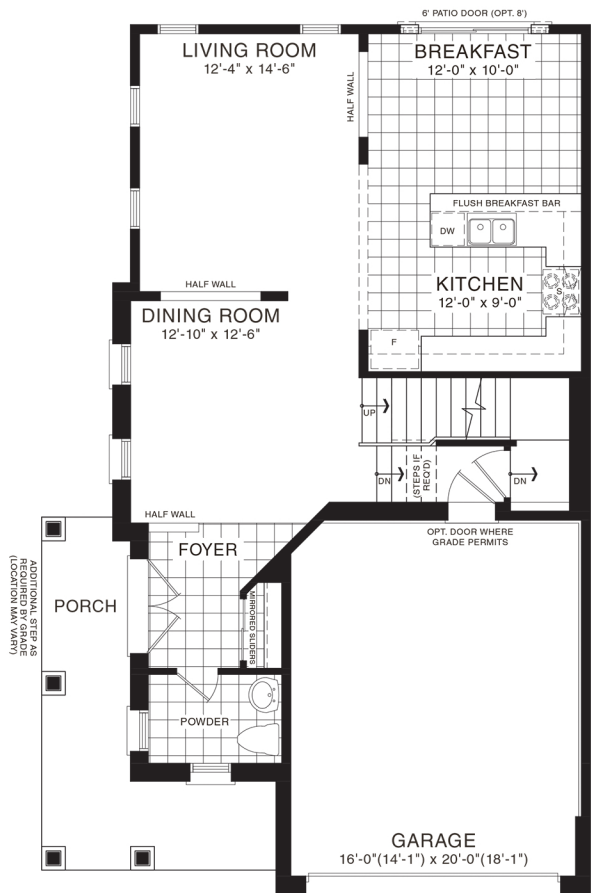
MAIN FLOOR PLAN STYLE A
